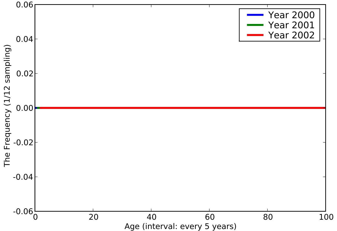
The Histogram of [Special screening for other rheumatic di], ACODE - [V822]
