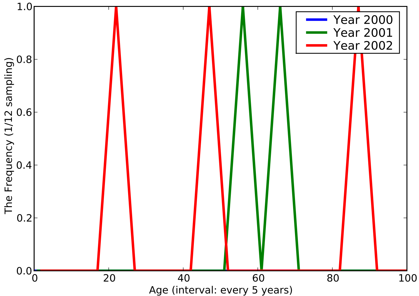
The Histogram of [Special screening for depression], ACODE - [V790]
