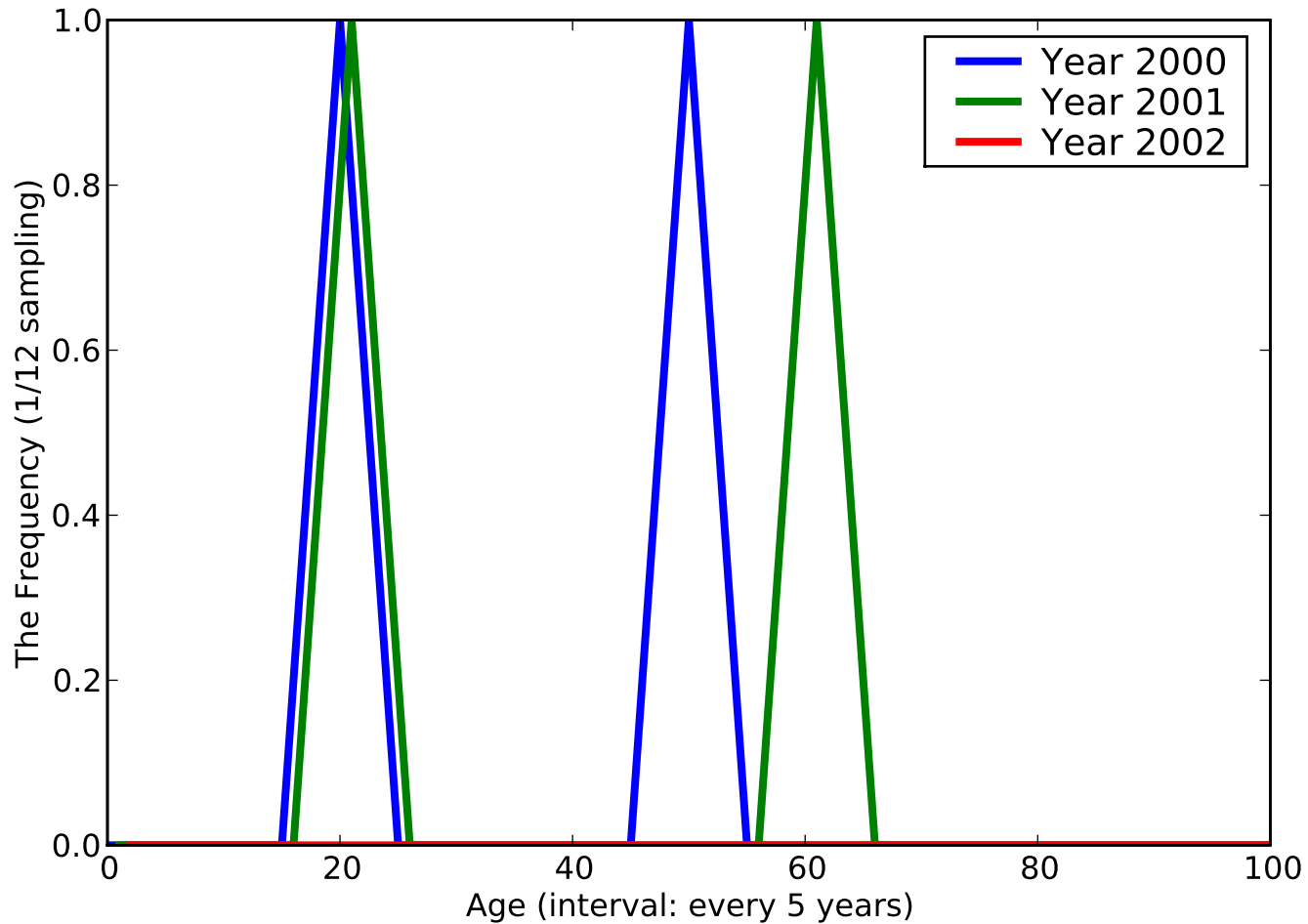
The Histogram of [Special screening examination for other ], ACODE - [V738]
