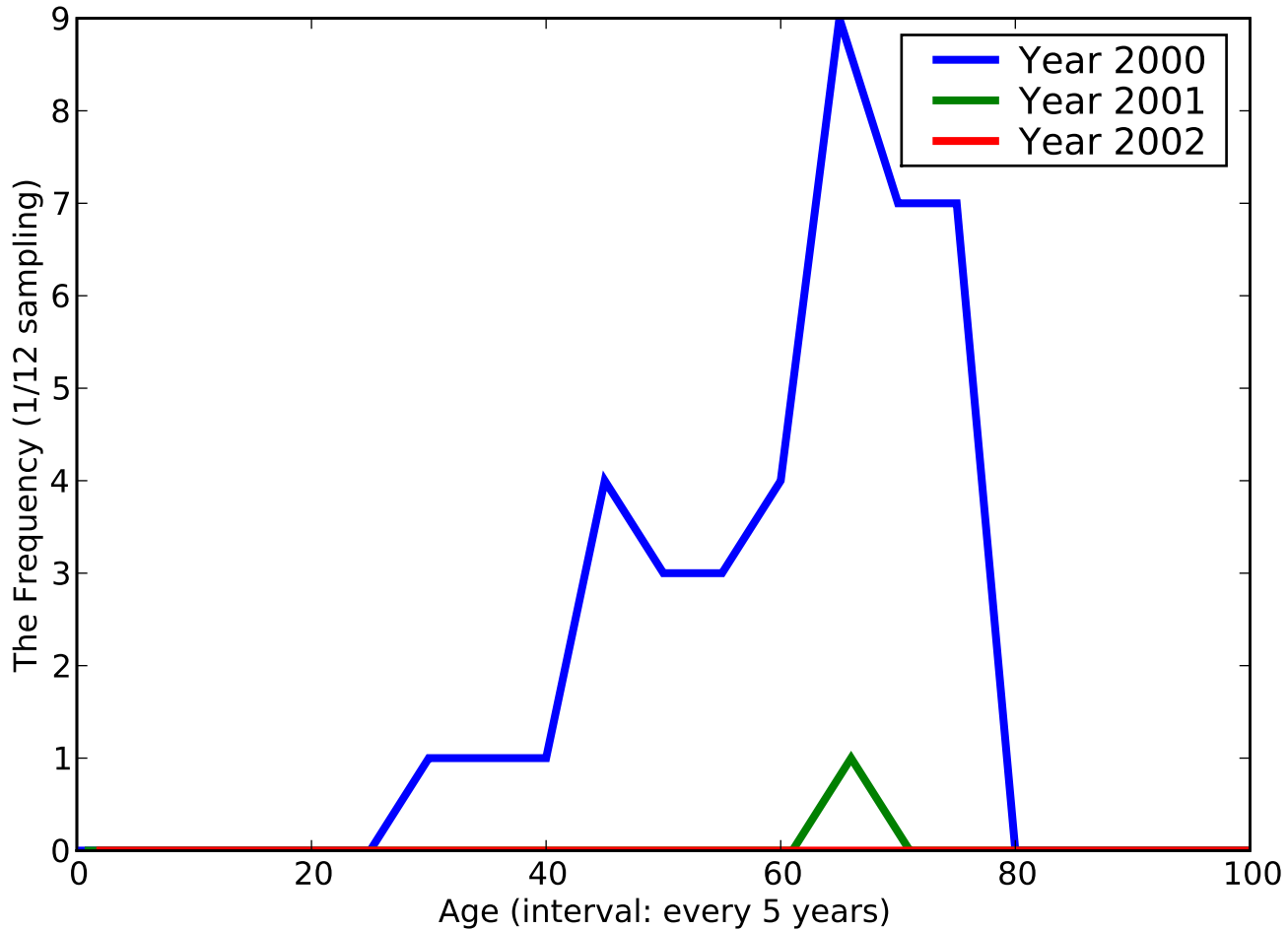
The Histogram of [Special investigations and examinations], ACODE - [V72]
