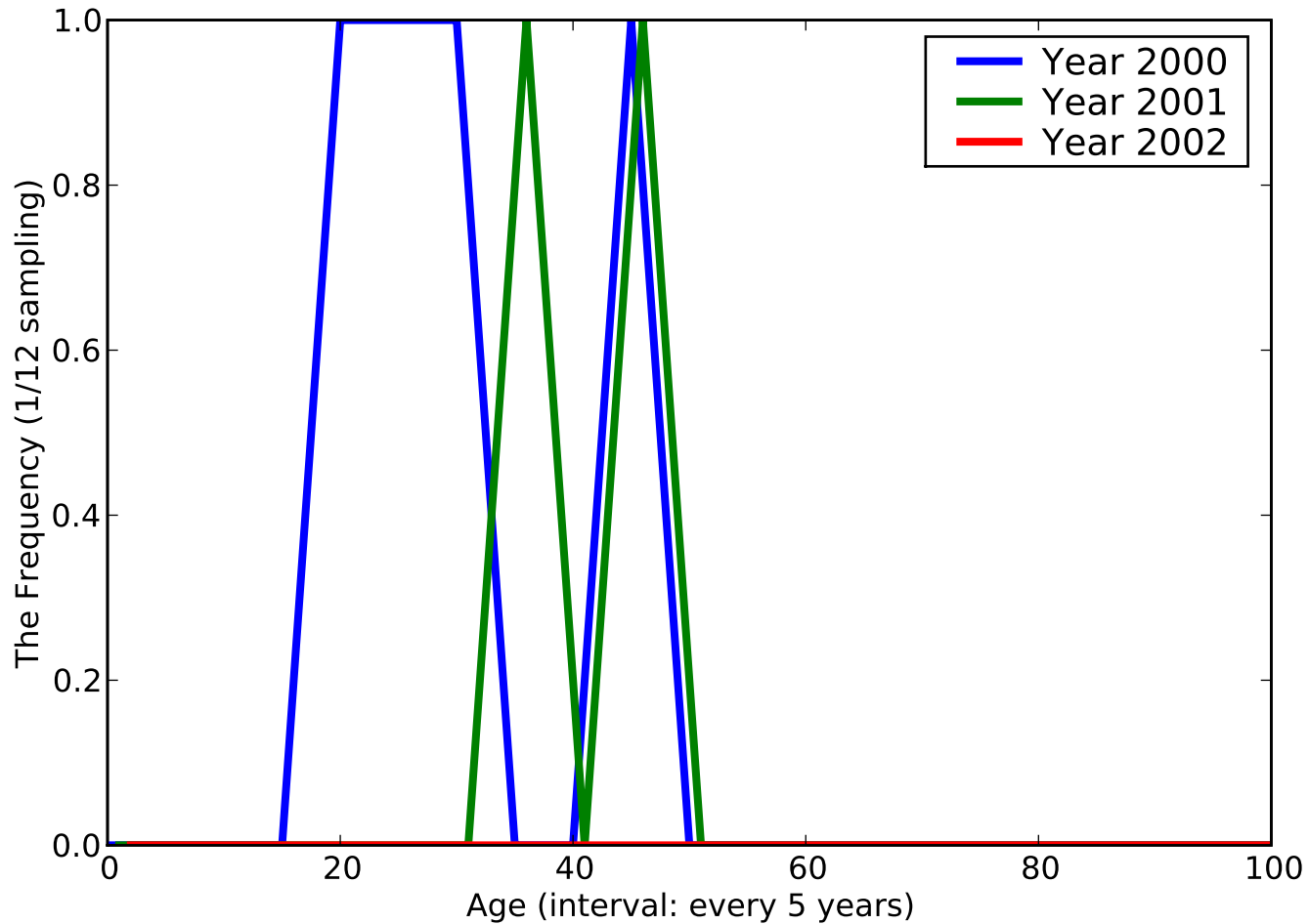
The Histogram of [Surveillance of previously prescribed co], ACODE - [V254]
