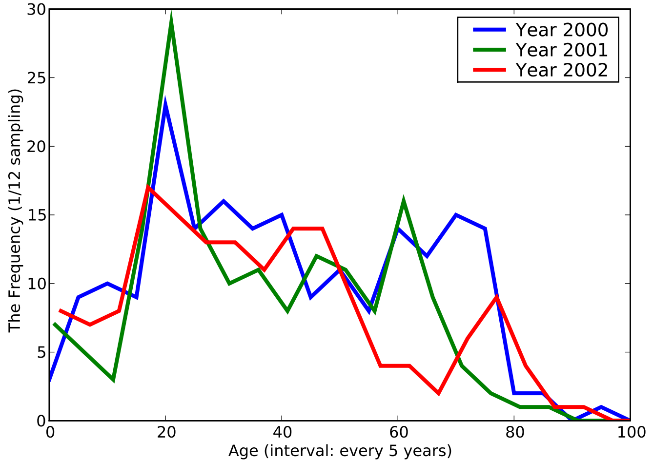
The Histogram of [Superficial injury of other multiple and], ACODE - [919]
