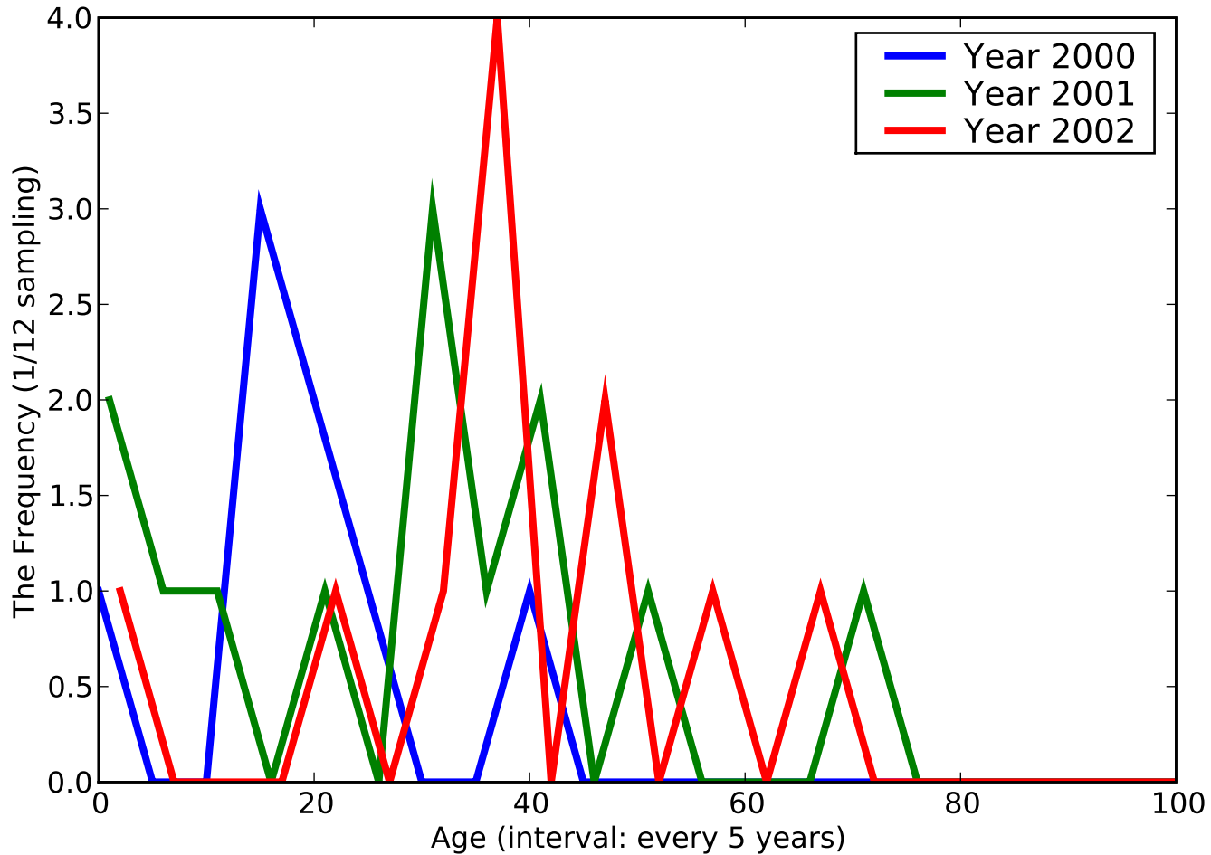
The Histogram of [Superficial injury of eye and adnexa], ACODE - [918]
