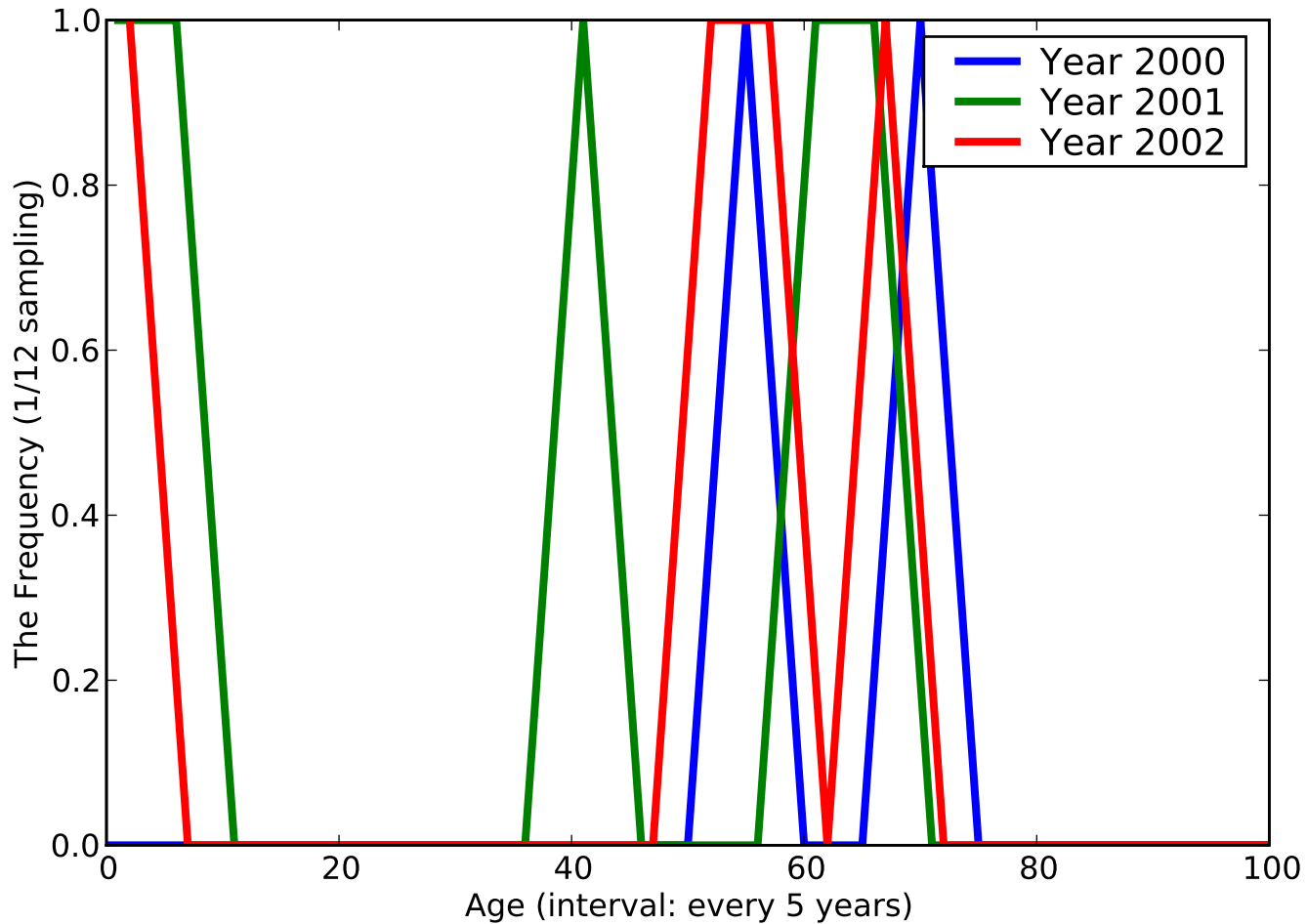
The Histogram of [Superficial injury of foot and toe(s) bl], ACODE - [9172]
