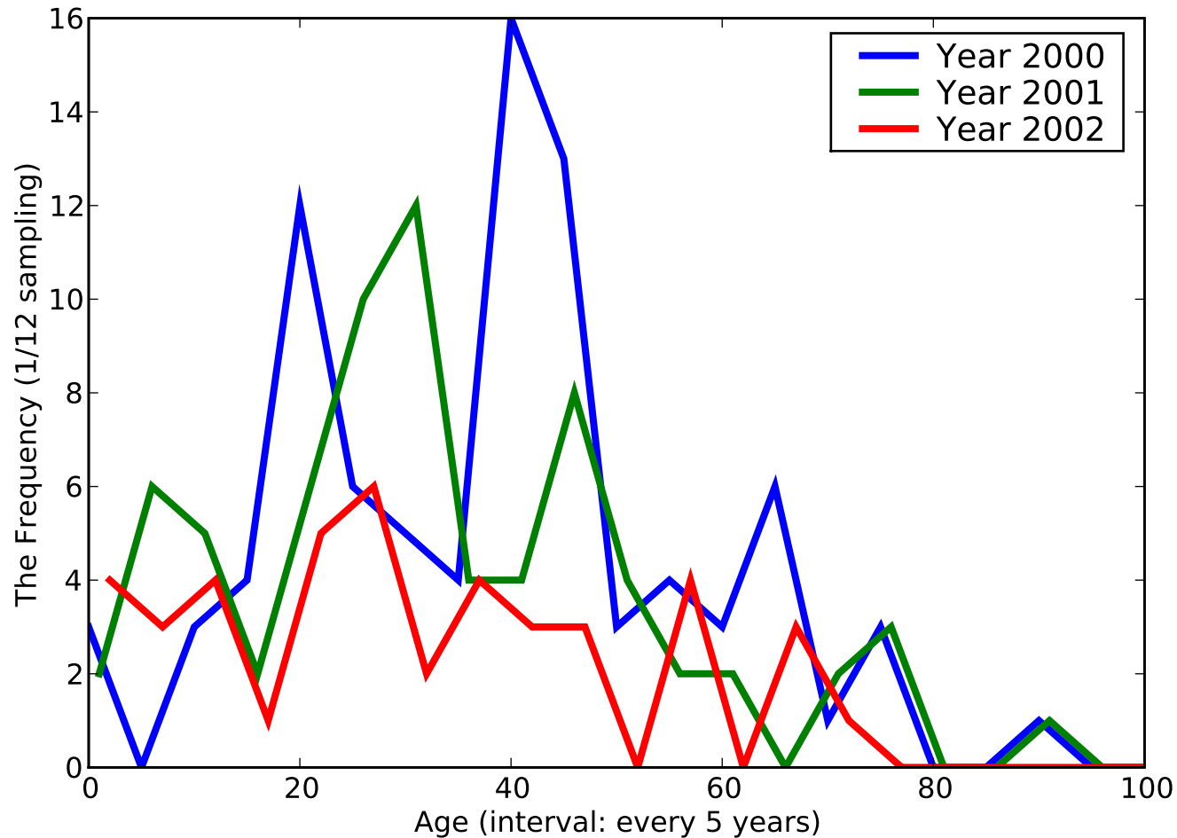
The Histogram of [Superficial injury of finger(s)], ACODE - [915]
