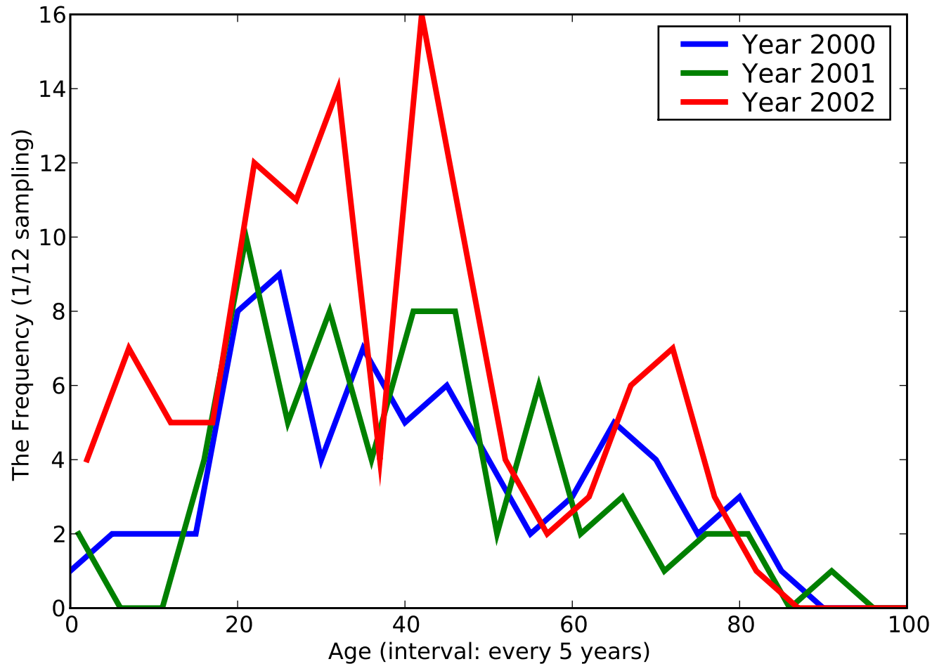
The Histogram of [Superficial injury of hand(s) except fin], ACODE - [9141]
