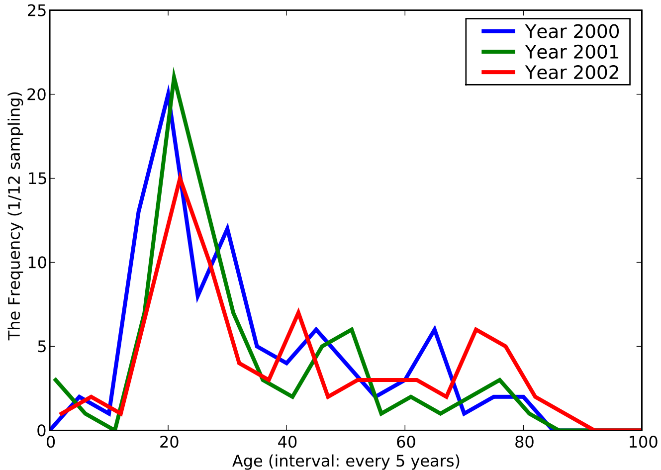
The Histogram of [Superficial injury of hand(s) except fin], ACODE - [914]
