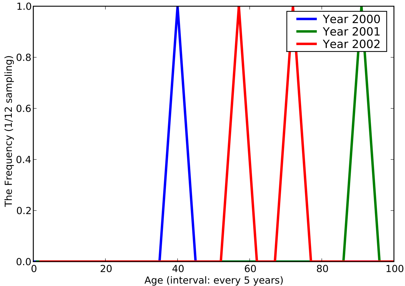
The Histogram of [Superficial injury of shoulder and upper], ACODE - [9123]
