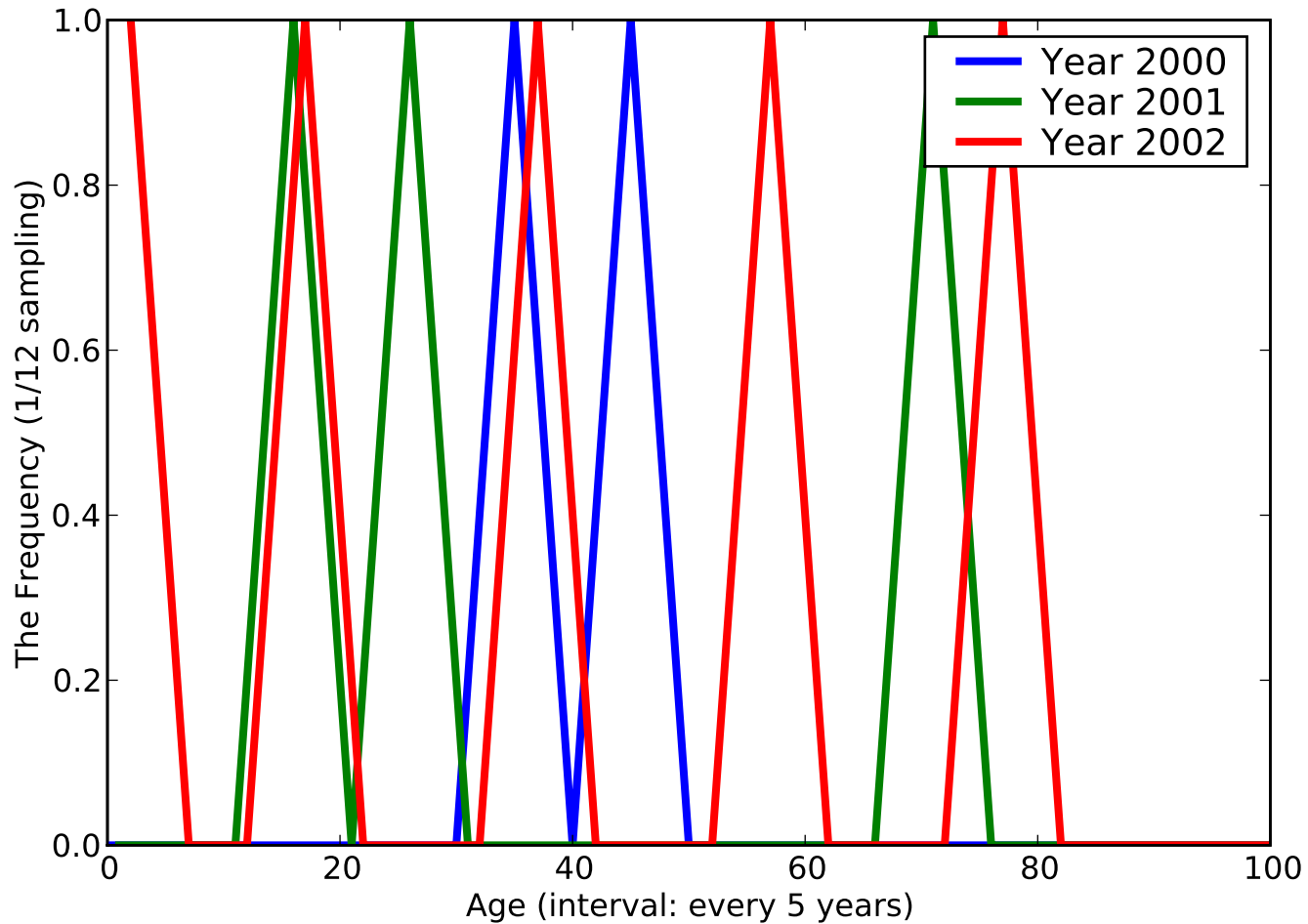
The Histogram of [Sprains and strains of sternoclavicular ], ACODE - [84841]
