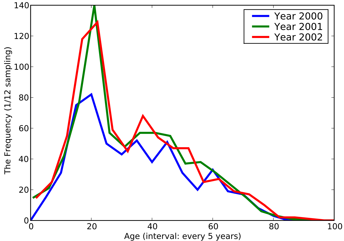
The Histogram of [Sprains and strains of other specified s], ACODE - [84509]
