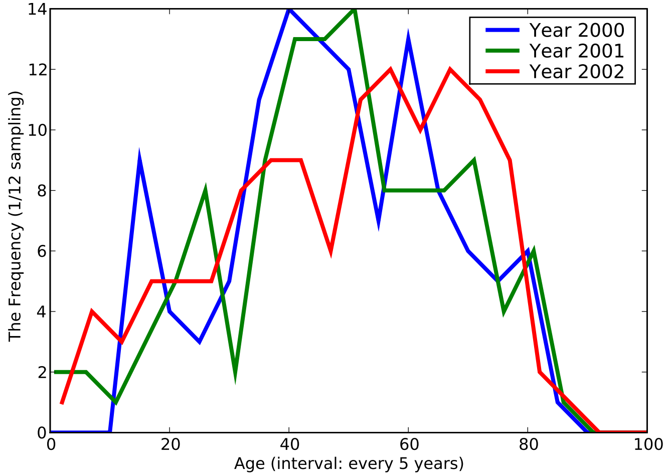
The Histogram of [Sprains and strains of other specified s], ACODE - [8438]
