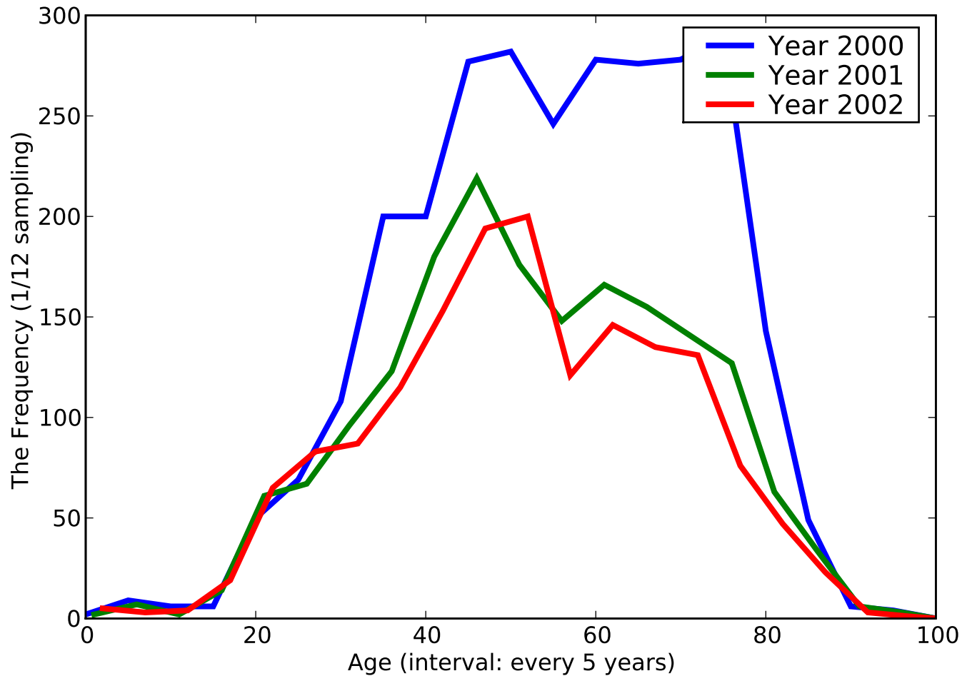
The Histogram of [Sleep disturbances], ACODE - [7805]
