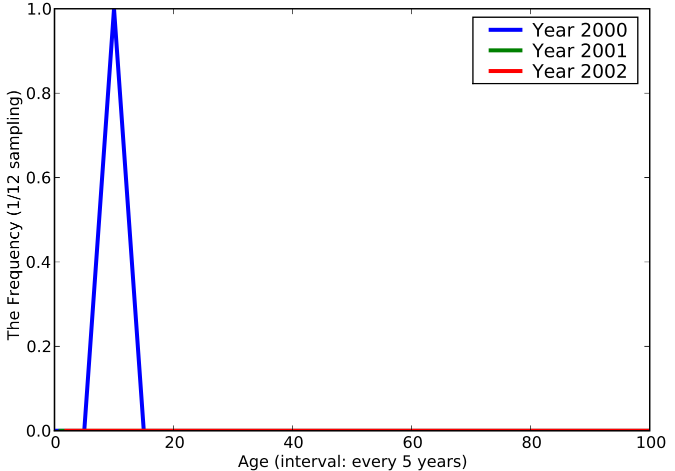
The Histogram of [Syndactyly of toes with fusion of bone], ACODE - [75514]
