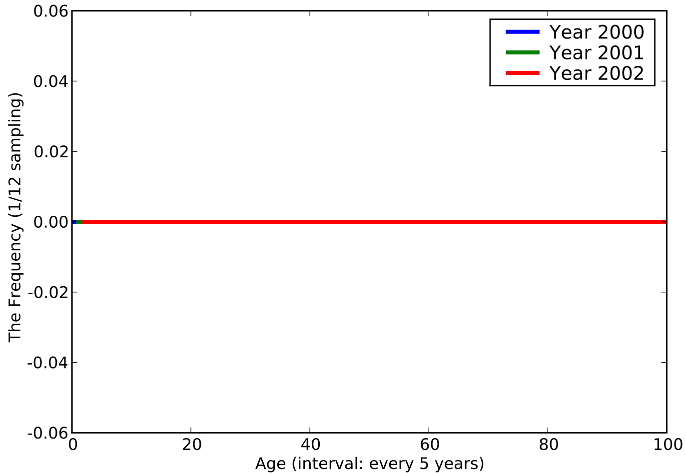
The Histogram of [Spina bifida without mention of hydrocep], ACODE - [74192]
