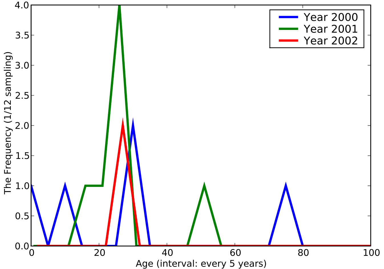
The Histogram of [Spina bifida], ACODE - [741]
