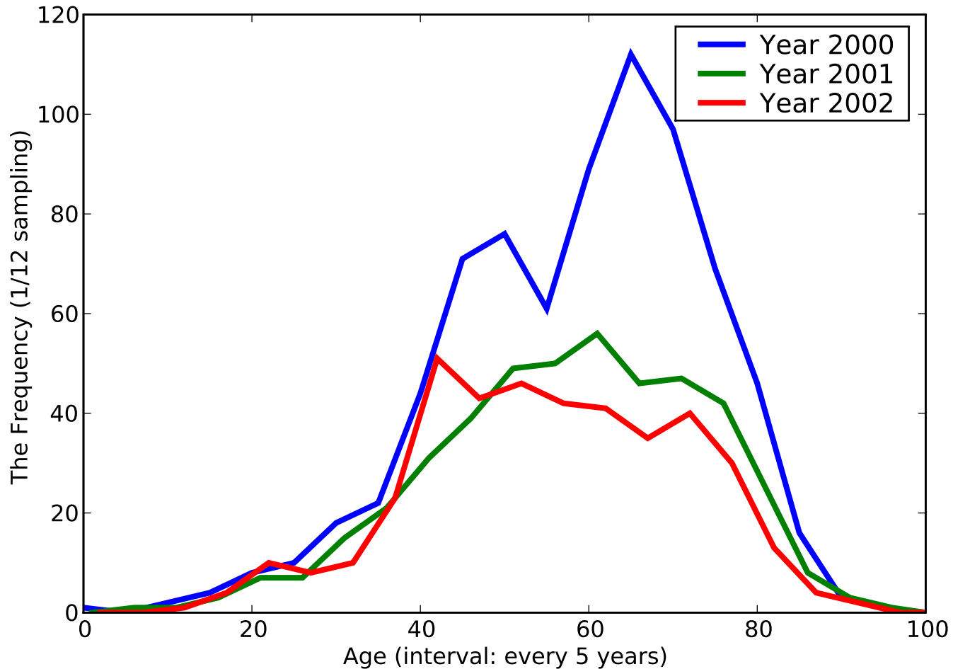
The Histogram of [Spondylosis and allied disorders], ACODE - [721]
