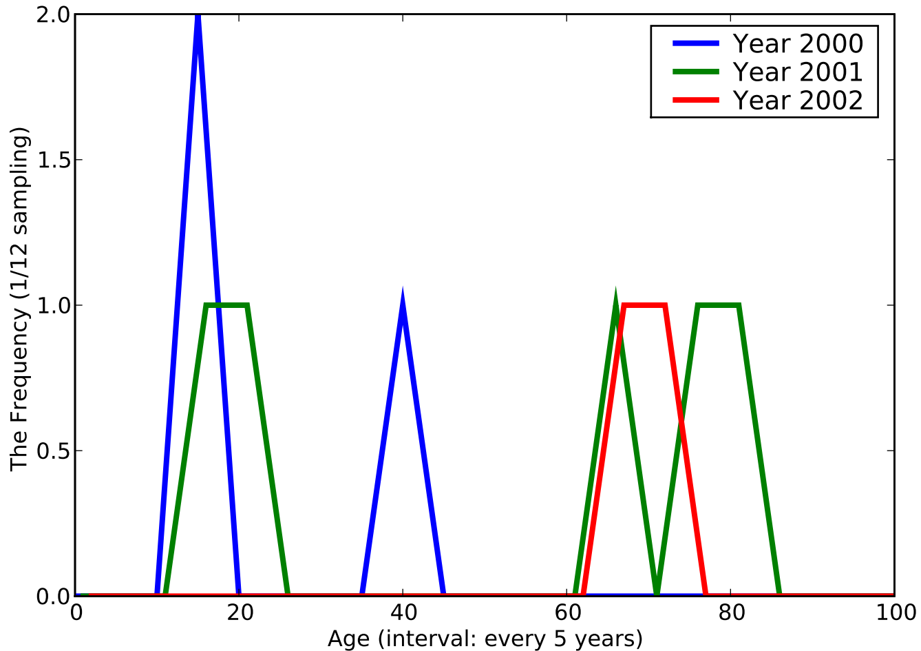
The Histogram of [Stiffness of joint not elsewhere classif], ACODE - [71959]
