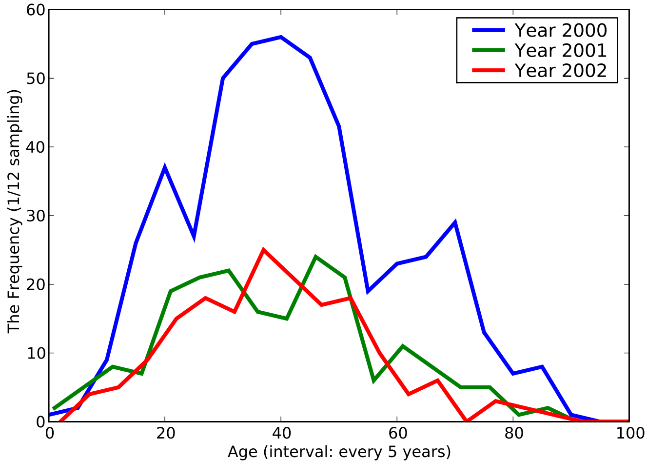
The Histogram of [Systemic lupus erythematosus], ACODE - [7100]
