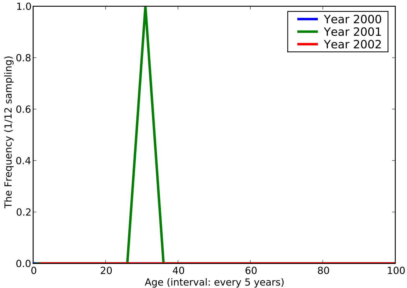
The Histogram of [Suspected damage to fetus from viral dis], ACode - [65533]
