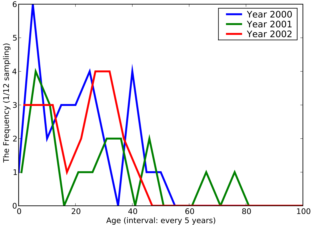
The Histogram of [Severe mental retardation], ACODE - [3181]
