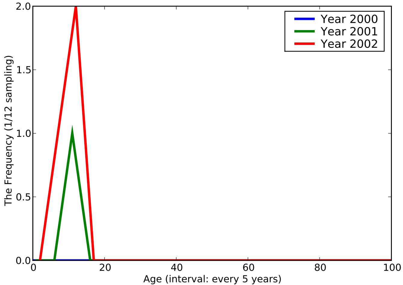
The Histogram of [Specific arithmetical disorder], ACODE - [3151]
