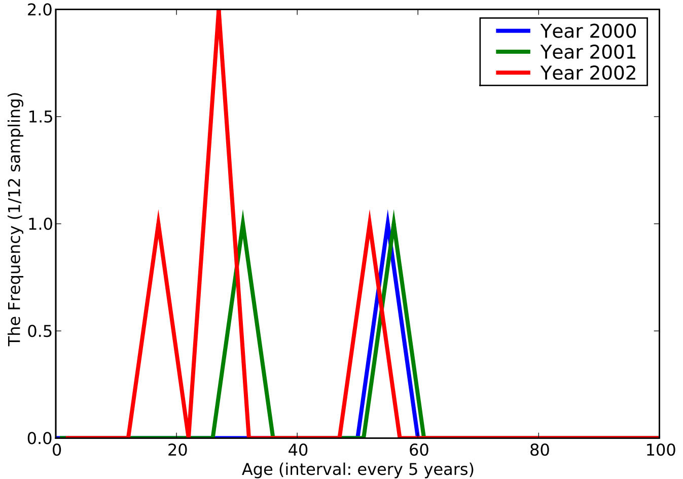
The Histogram of [Schizoid personality disorder unspecifie], ACODE - [30120]
