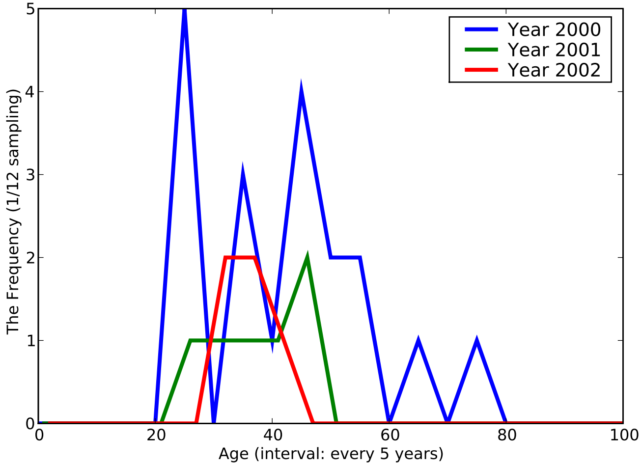
The Histogram of [Schizophrenic disorders paranoid type in], ACODE - [29535]
