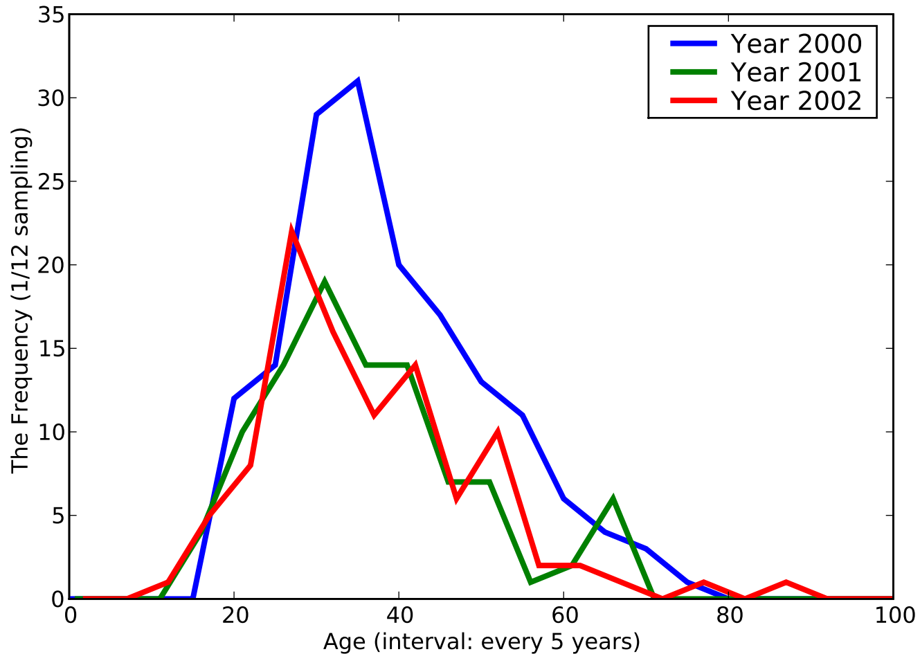
The Histogram of [Schizophrenic disorders paranoid type un], ACODE - [29530]
