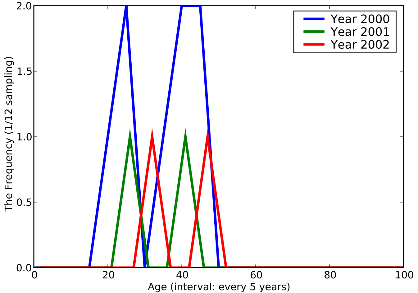
The Histogram of [Schizophrenic disorders catatonic type u], ACODE - [29520]
