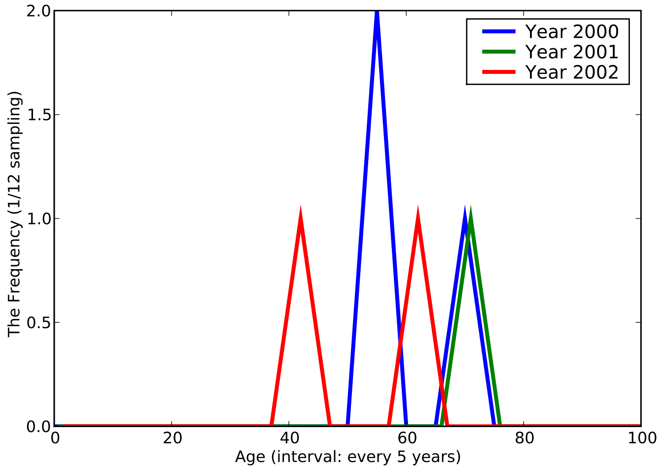
The Histogram of [Secondary malignant neoplasm of other re], ACODE - [1973]
