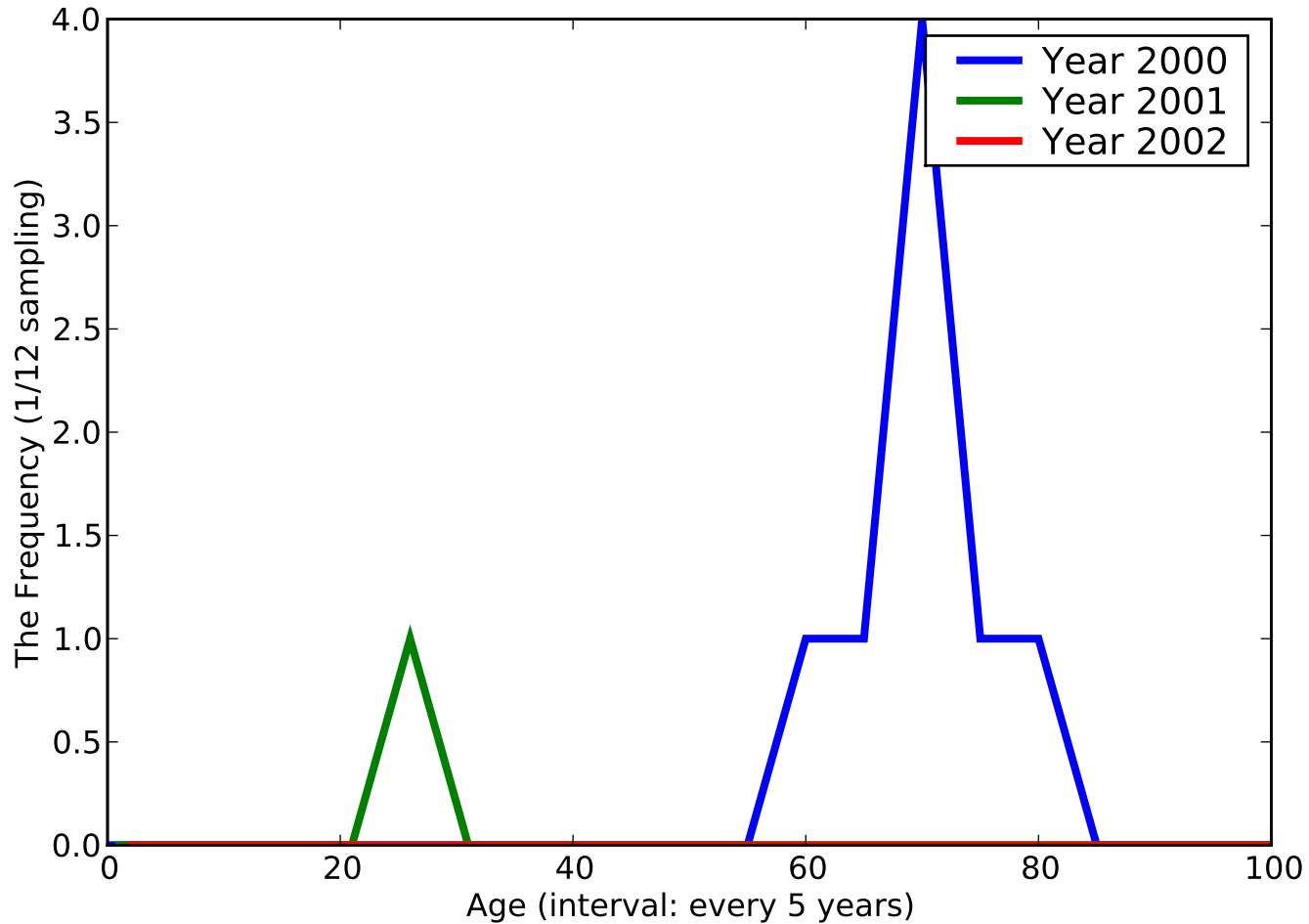
The Histogram of [Sarcosporidiosis], ACODE - [1365]
