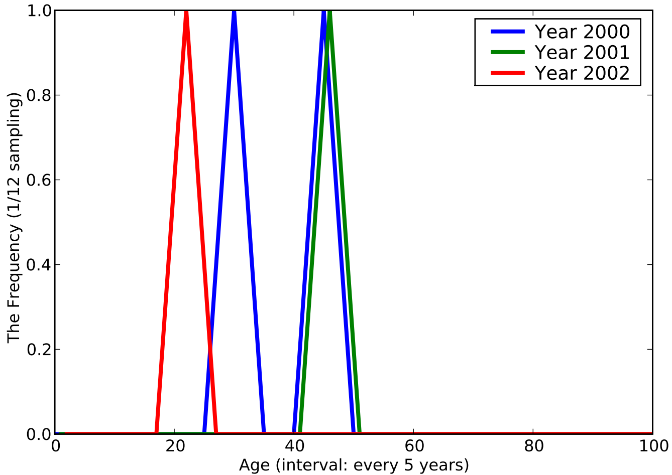
The Histogram of [Sarcoidosis], ACode - [135]
