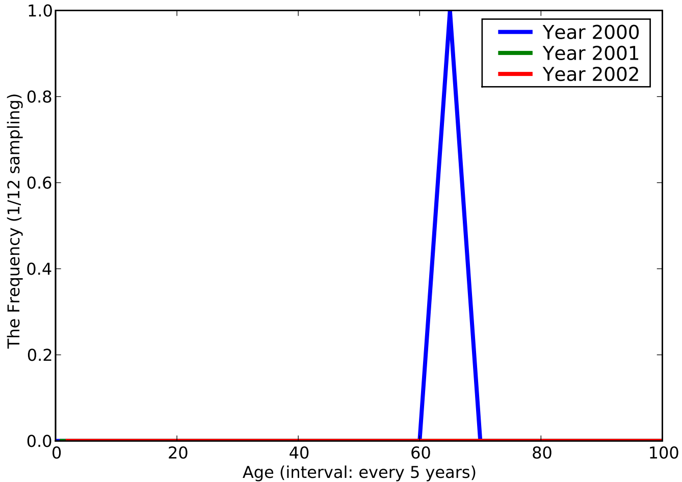
The Histogram of [Sporotrichosis], ACODE - [1171]
