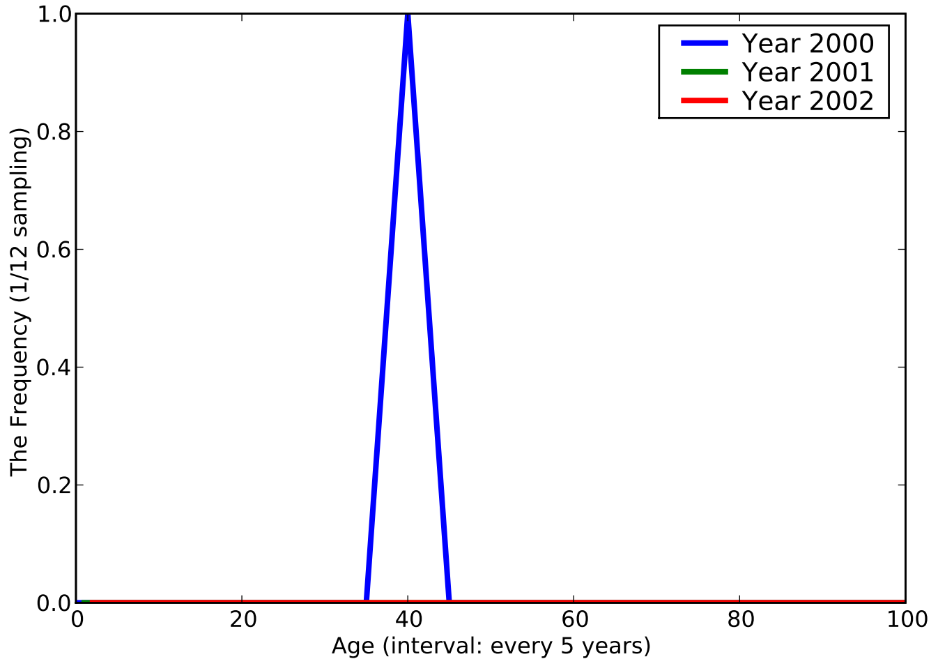
The Histogram of [Syphilis of liver], ACODE - [0953]
