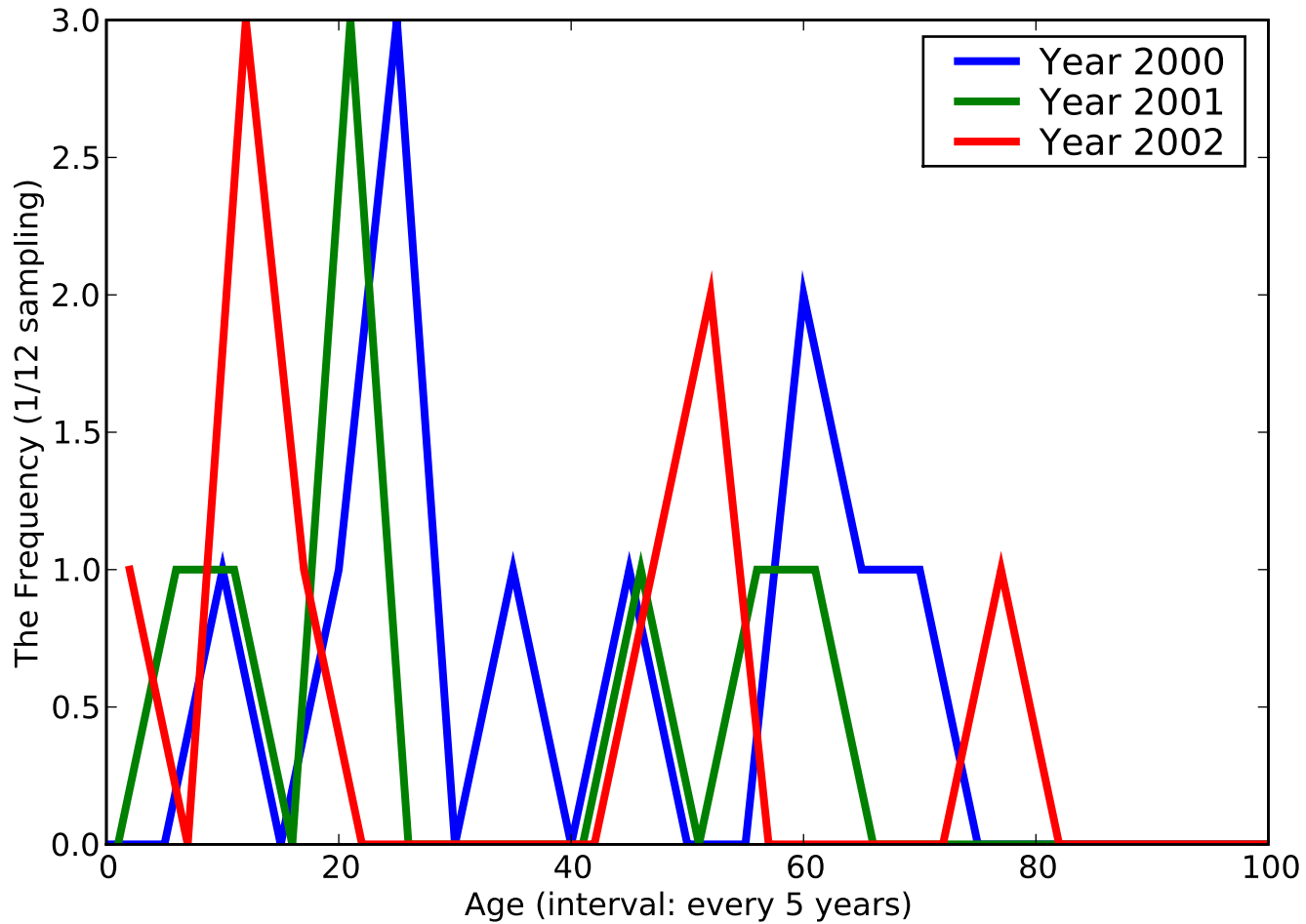
The Histogram of [Spotted fevers], ACODE - [0820]
