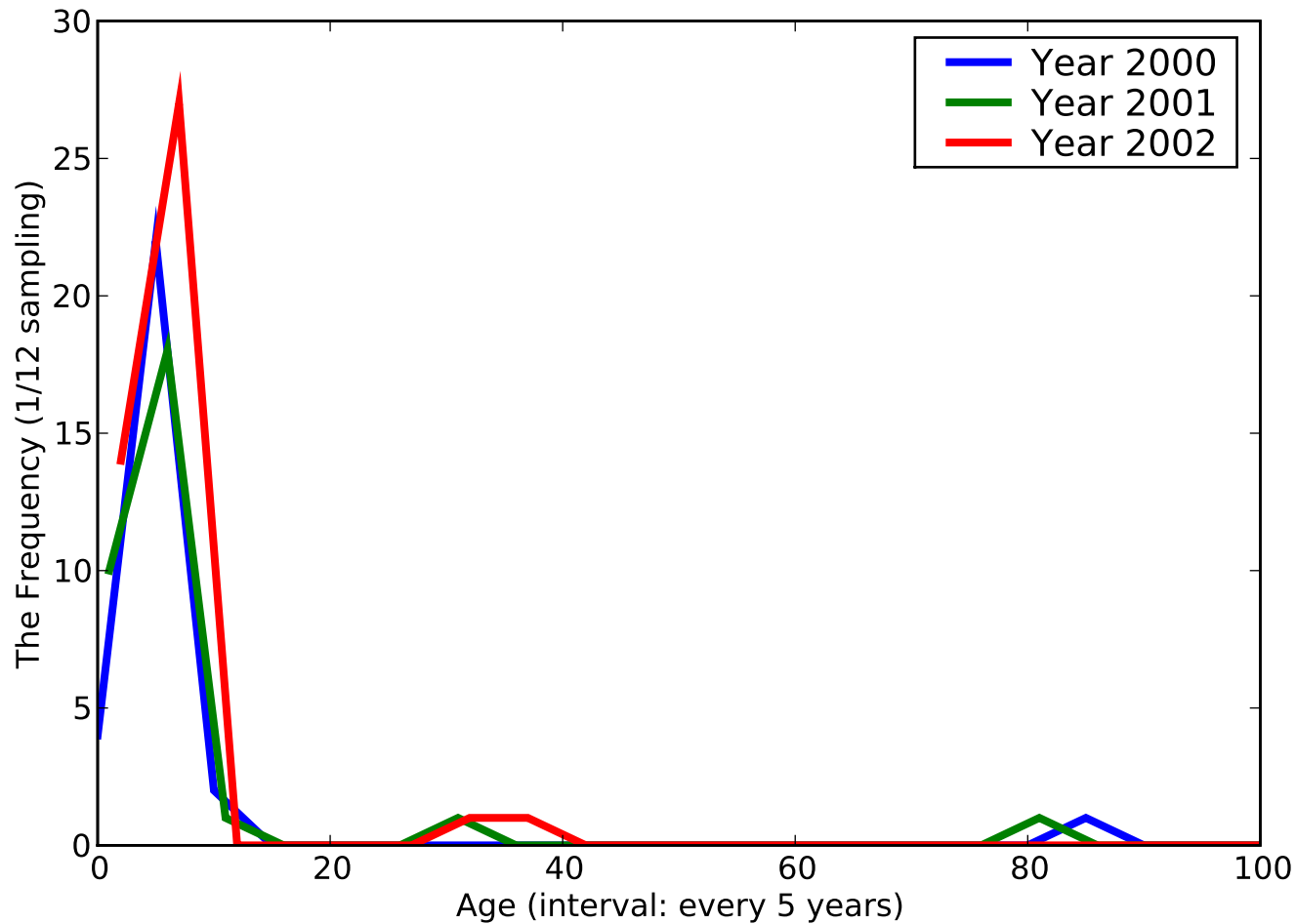
The Histogram of [Scarlet fever], ACode - [0341]
