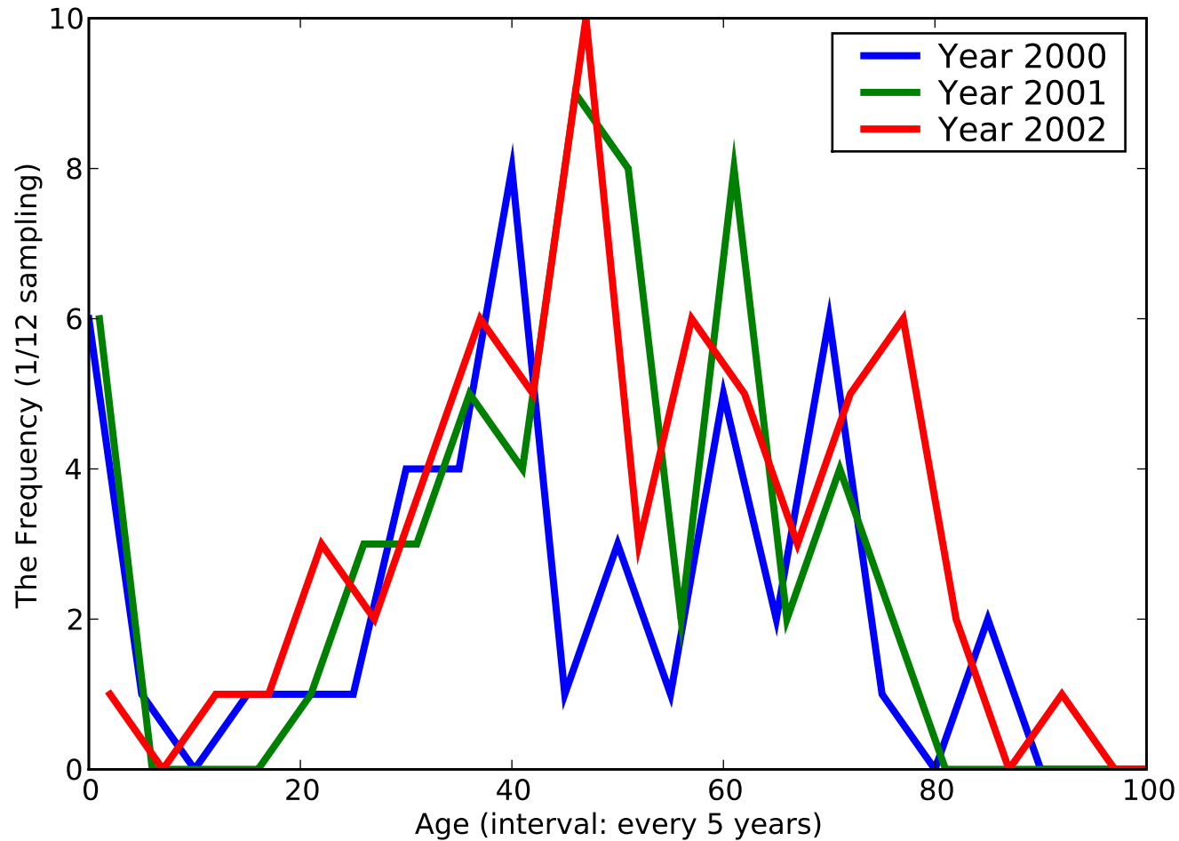
The Histogram of [Hepatomegaly], ACODE - [7891]
