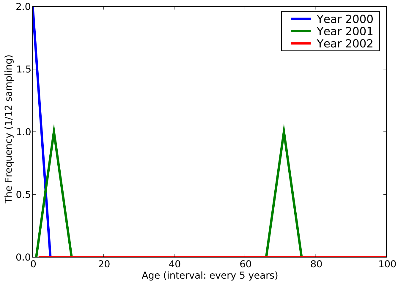
The Histogram of [Hemolytic disease due to other and unspe], ACODE - [7732]
