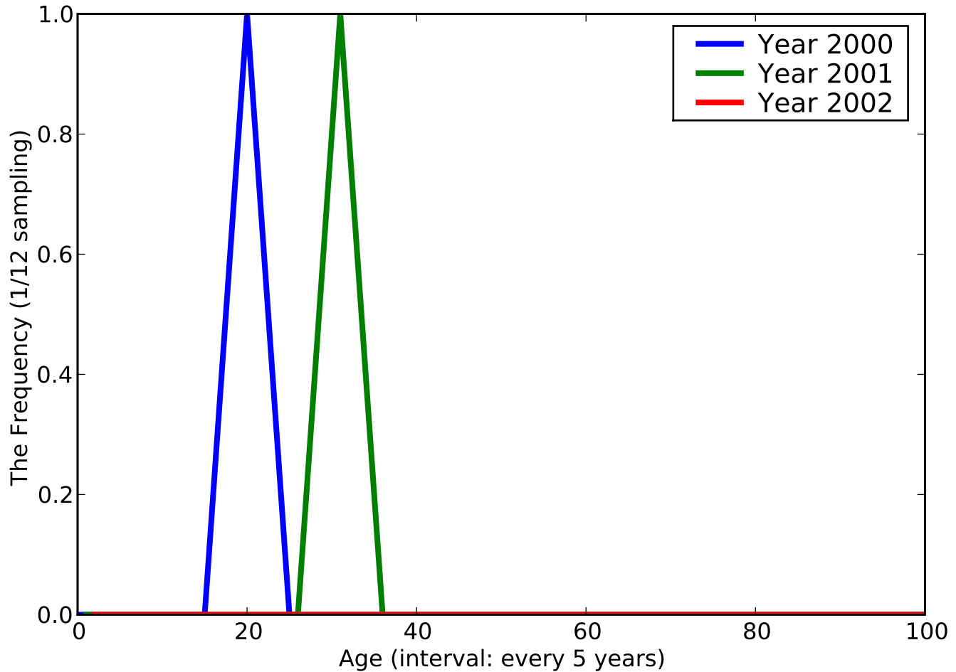
The Histogram of [High vaginal laceration], ACode - [6654]
