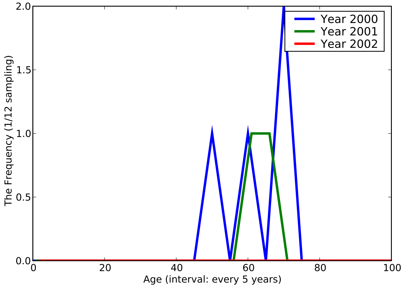
The Histogram of [Hyperplasia of prostate unspecified], ACODE - [6009]
