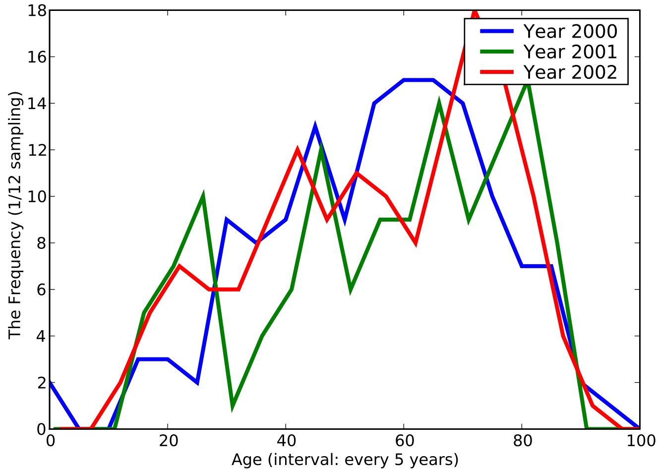
The Histogram of [Hypotension unspecified], ACODE - [4589]
