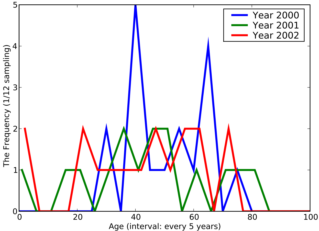
The Histogram of [Hemangioma other sites], ACODE - [22809]
